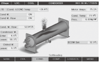
State of condenser
