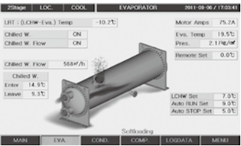
State of evaporator
